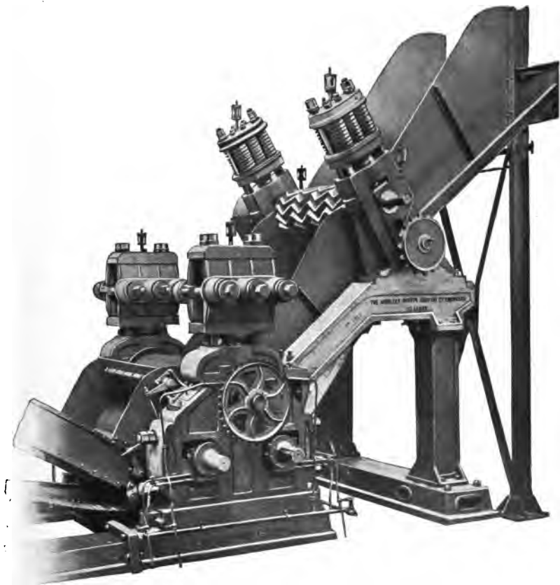
FIG. 7. KRAJEWSKI CRUSHER AND FIRST MILL-UNIT.
